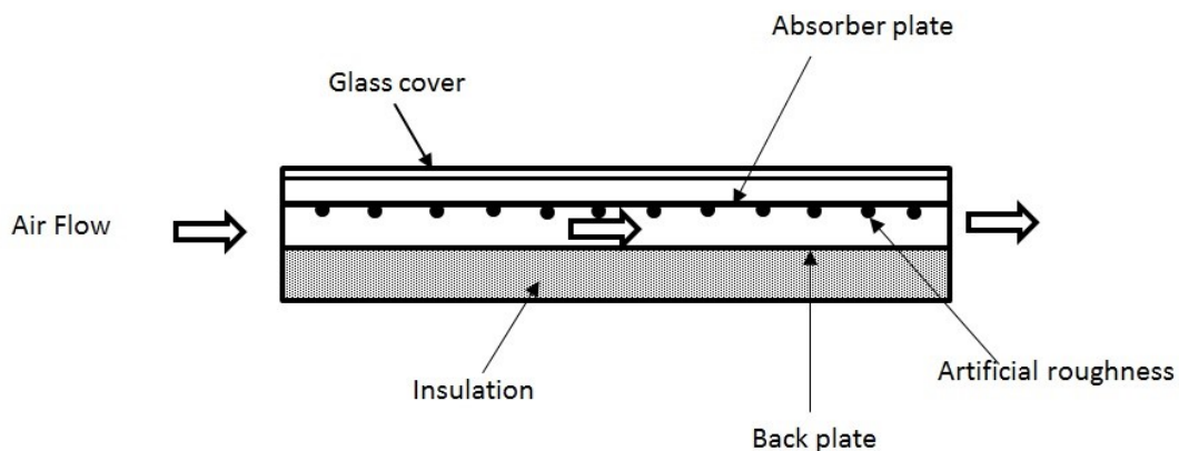
Figure 2. Test section
